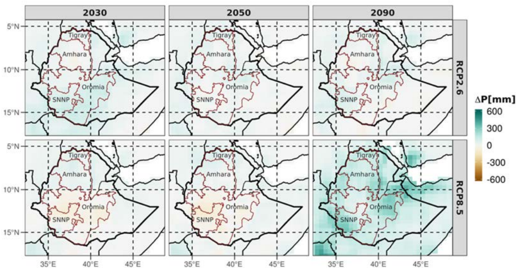
Figure 11: Annual average precipitation difference in 2030, 2050 and 2090 in relation to 2007 under RCP2.6 (top) and RCP8.5 (bottom) projected by the multi-model mean.
