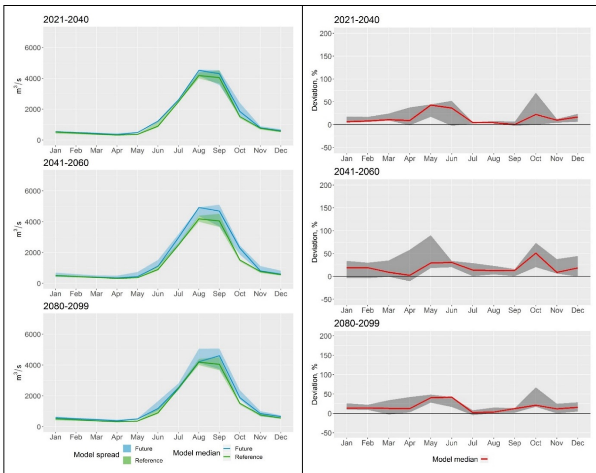
Figure 16: Absolute (left) and relative (right) mean monthly discharge changes of the river discharge at the Sudan border gauge (Blue Nile basin) for three future periods, compared to the reference period under RCP2.6.
