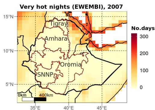
Figure 9: Average number of tropical nights (temperature above 25°C) per year in 2007, as indicated by EWEMBI.
