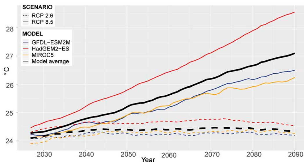
Figure 6: Projected mean annual temperature over Ethiopia for two scenarios and three climate models. The graph shows the 20-year moving average.
