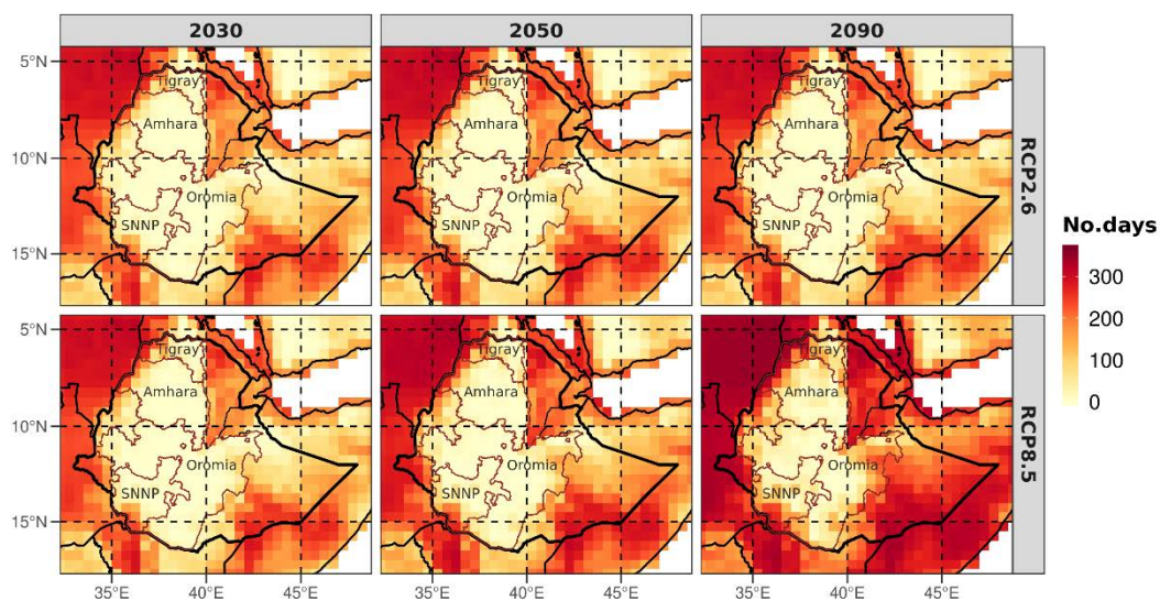
Figure 8: Average number of very hot days (temperature above 35°C) per year in 2030, 2050 and 2090 under scenario RCP2.6 and RCP8.5. Results are averages over the three ISIMIP models.
