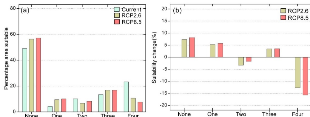
Figure 28: Suitability of multiple crops in Ethiopia under current and projected climatic conditions.
