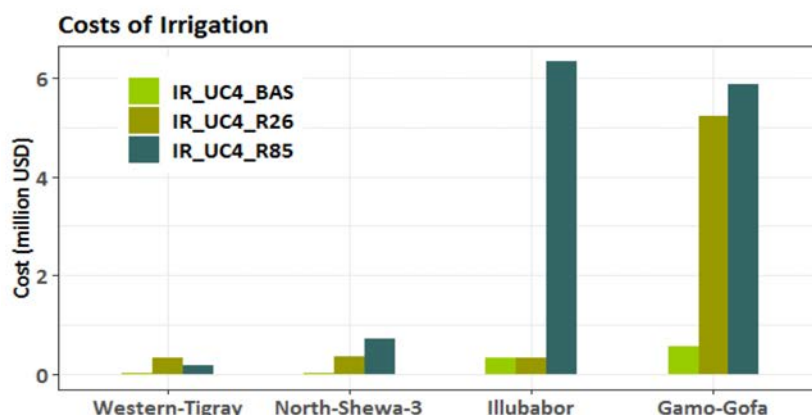
Figure 48: Costs of irrigation (IR) associated with high unit costs (UC 4 = 298 USD/ha/meher) in the baseline (BAS), under RCP2.6 (R26), and under RCP8.5 (R85).
