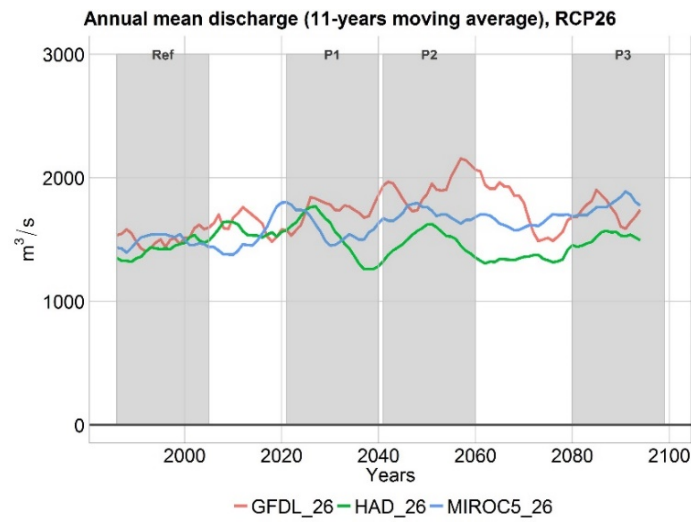
Figure 14: Annual mean discharge at the Sudan border gauge (11-years moving average) under RCP2.6.
