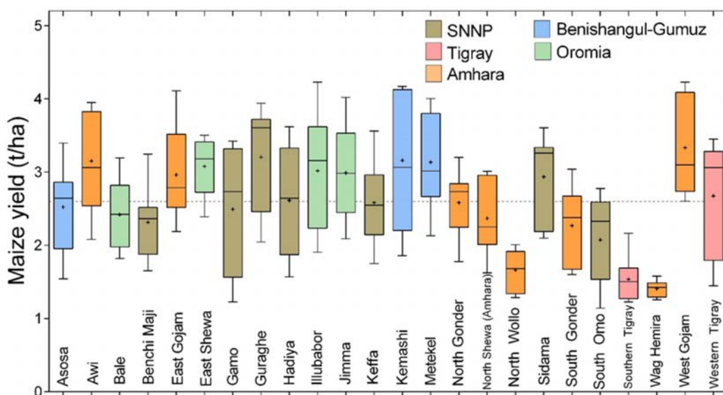
Figure 20: Current observed trends in maize yield for each zone. The dotted line is the long-term national maize yield average.
