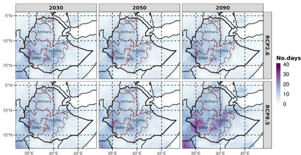
Figure 12: Number of days with heavy precipitation per year under scenarios RCP2.6 (top) and RCP8.5 (bottom) for 2030 (left), 2050 (middle) and 2090 (right), projected by the ISIMIP multi-model mean.
