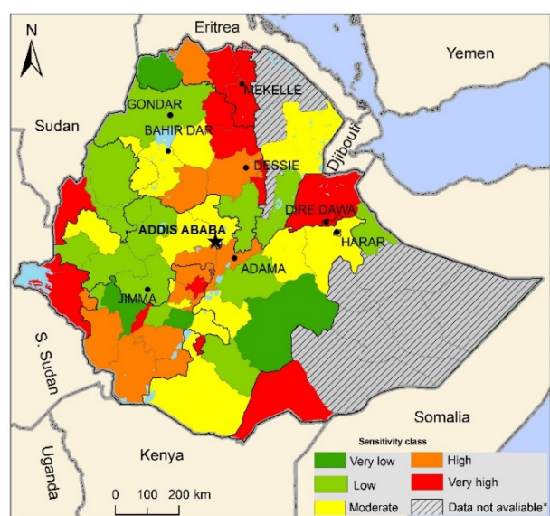
Figure 41: Spatial distribution of the sensitivity index showing the five classes at zone level.
