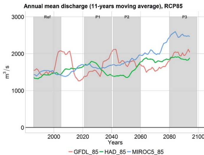
Figure 15: Annual mean discharge at the Sudan border gauge (11-years moving average) under RCP8.5.
