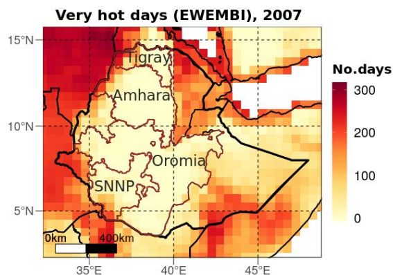
Figure 7: Average number of very hot days (temperature above 35°C) per year in 2007, as indicated by EWEMBI.
