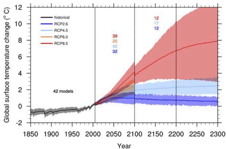
Figure 3: Multi-model mean global annual mean surface air temperature (relative to 1986-2005) for each RCP (IPCC, 2014a).
