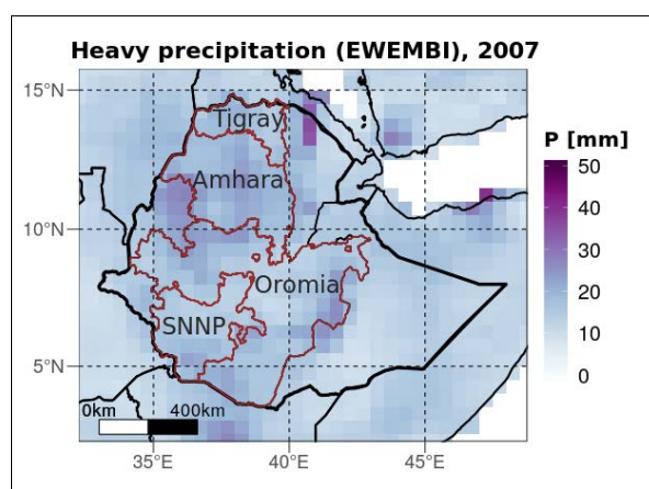
Figure 5: Daily heavy precipitation extreme threshold in 2007 (average 16.6 mm over the whole of Ethiopia) (EWEMBI).
