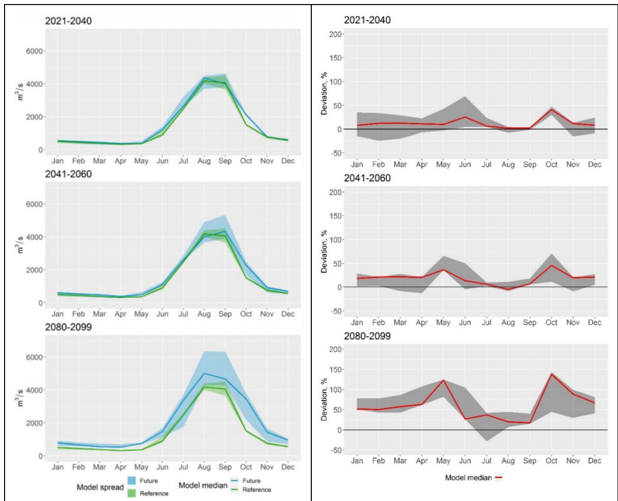
Figure 17: Absolute (left) and relative (right) mean monthly discharge changes of the river discharge at the Sudan border gauge (Blue Nile basin) for three future periods compared to the reference period under RCP8.5.
