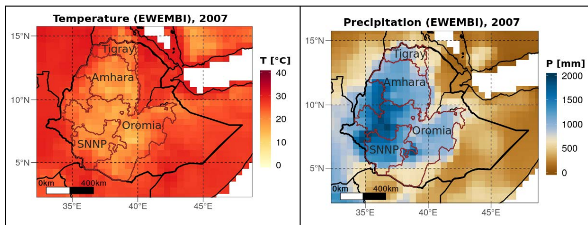
Figure 4: Mean annual temperature (left) and annual precipitation sum (right) in 2007 (1997-2016) over Ethiopia.
