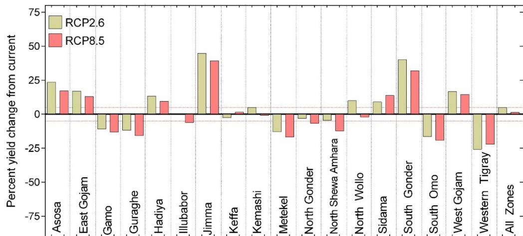
Figure 21: Climate change induced yield changes for selected zones in Ethiopia under the RCP2.6 and RCP8.5 scenarios, without CO 2 fertilisation. The red dotted lines represent the 10% window within which yield changes are considered stable.
