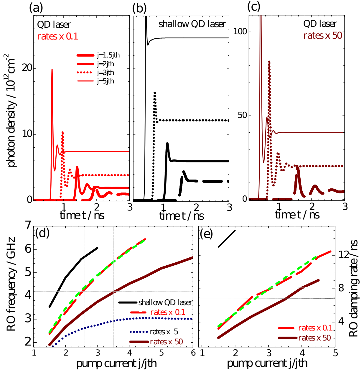
FIG. 3. Turn-on oscillations for QD lasers with three different internal carrier-scattering lifetimes: (a) 10-fold slower rates than microscopically calculated, (b) rates as obtained for shallow dot QD laser, (c) 50-fold faster rates. The pump current varies between j = 1.5j_{th} and j = 5j_{th} (note that the threshold current changes with \tau ). (d) and (e) show the RO frequency and damping rates, respectively, in terms of the pump current as obtained by fitting the turn-on dynamics plotted above close to the fixed point. Green dashed lines: Analytic results for 10-fold slower rates given by Eqs. (7), (8).
