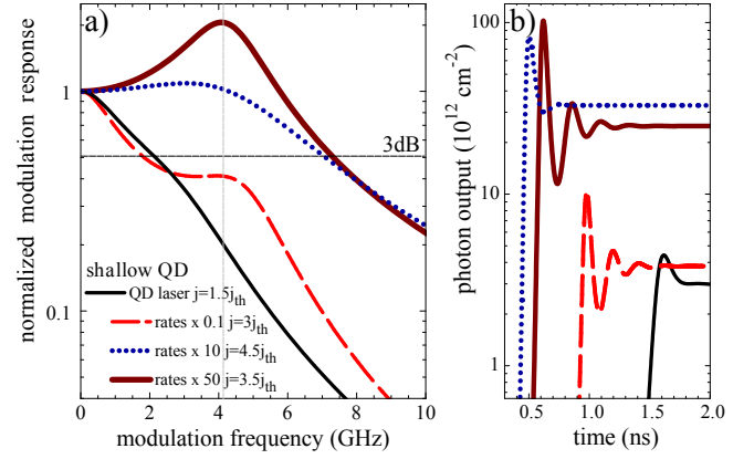
FIG. 4. (a) Electrical modulation response of a quantum dot laser and (b) corresponding turn-on dynamics with the different internal scattering lifetimes already used in Fig. 3. The pump current was chosen to yield equal RO frequency for all 4 lasers (see thin horizontal line in Fig. 3d).
