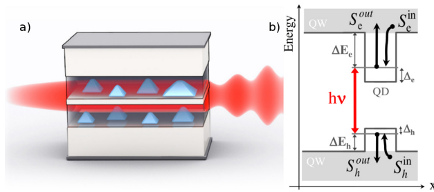
FIG. 1. (a) Scheme of the optically injected QD laser. QDs (light blue pyramids) are surrounded by a quantum well (QW) (b) Energy diagram of the band structure across a QD. h\nu labels the ground state (GS) lasing energy. \Delta E_e and \Delta E_h mark the energetic distance of the GS from the QW band edge for electrons and holes, respectively. \Delta_e and \Delta_h denote the distance to the bottom of the QD confinement potential.
