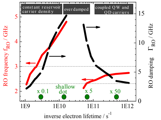
FIG. 2. Turn-on damping \Gamma_{RO} and relaxation oscillation frequency f_{RO} of a QD laser with different internal steady state scattering lifetimes. The green circles denote the different QD lasers discussed in the following. The pump current is set to j = 2j_{th} (note that the threshold current j_{th} changes with \tau )
