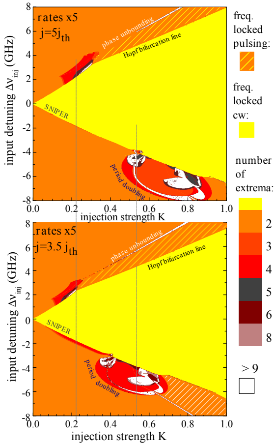
FIG. 6. Locking tongues of a shallow-dot QD laser with 5-fold faster rates for two different electrical pump currents j = 3.5j_{th} and j = 5j_{th} . Colored shading labels the number of maxima found in the time series per period, and yellow shading shows the locking region.
