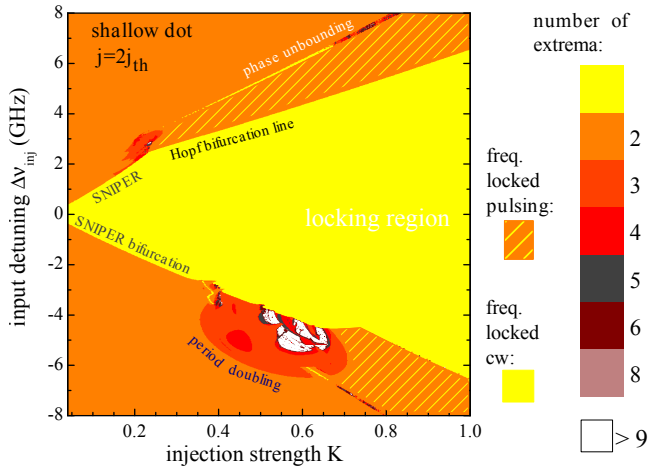
FIG. 5. Two-parameter bifurcation diagram of the shallow-dot QD laser introduced above. Colored shading labels the number of maxima found in the time series per period, and the yellow shading shows the region of cw laser emission (locking tongue).
